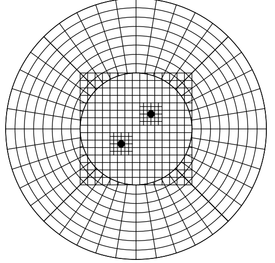
FIG. 1: Schematic diagram of a typical Llama grid setup in the (x, y) plane. Note the inner Cartesian grid with box-in-box AMR which is joined to a 6-patch multiblock structure (only 4 of these patches are shown in the (x, y) plane).
