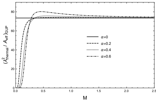
FIG. 2. GUP-corrected dimensionless parameter \frac{\lambda_{thermal}^2}{A_{eff}}|_{GUP} as given by (28) versus M for different values of \alpha . We have taken natural units c = G = \hbar = 1
