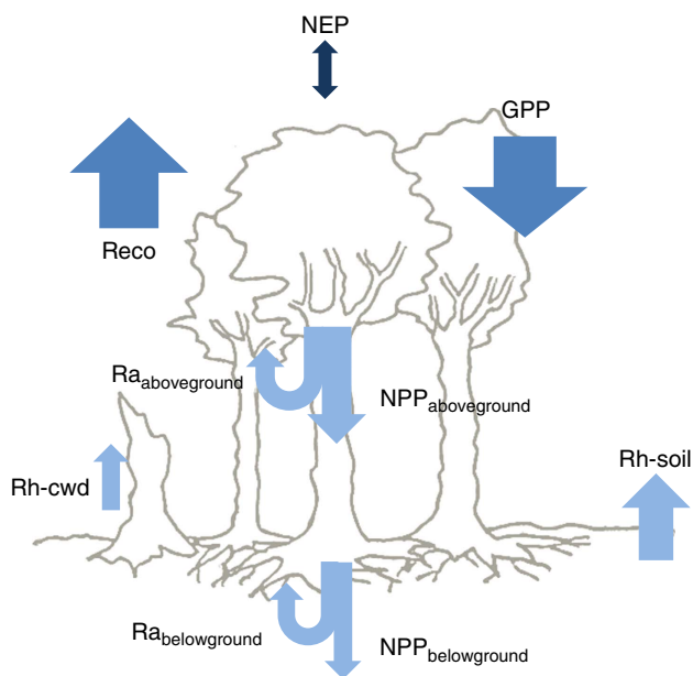
Figure 1 | Schematic representation of the major components of the forest carbon cycle. Ra aboveground and Ra belowground : above- and below-ground autotrophic respiration, respectively (their sum is indicated as Ra); Rh-soil and Rh-cwd: heterotrophic respiration from soil and coarse woody debris, respectively (their sum is indicated as Rh); NPP aboveground and NPP belowground : above- and belowground net primary production, respectively (their sum is indicated as NPP); Reco: ecosystem respiration (Reco = Ra + Rh); GPP: gross primary production (GPP = NPP + Ra), and NEP: net ecosystem production (NEP = GPP – Reco = NPP – Rh). Each flux is associated with an arrow. Arrows pointing down indicate carbon (C) uptake, arrows pointing up indicate C release, whereas the up-down arrow indicates that both C release and C uptake can occur. The dark blue arrow indicates NEP, the mid-blue arrows indicate the primary components of NEP (Reco and GPP), whereas the light blue arrows indicate the components of Reco and GPP.
