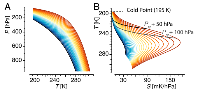
Fig. 5. (A) Vertical profile of temperature (plotted as a function of pressure) and (B) static stability (plotted as a function of atmospheric temperature) computed by assuming that the atmosphere follows a moist adiabat starting at 950 hPa and associated with a range of cloud-base temperatures (increasing from blue to red). The dashed lines in B show a constant pressure distance (50 hPa and 100 hPa) from the cold point tropopause. Above these levels, the static stability of the actual atmosphere significantly deviates from a moist-adiabatic stratification and increases up to the tropopause, the moist-adiabatic assumption thus representing a lower bound on static stability.
