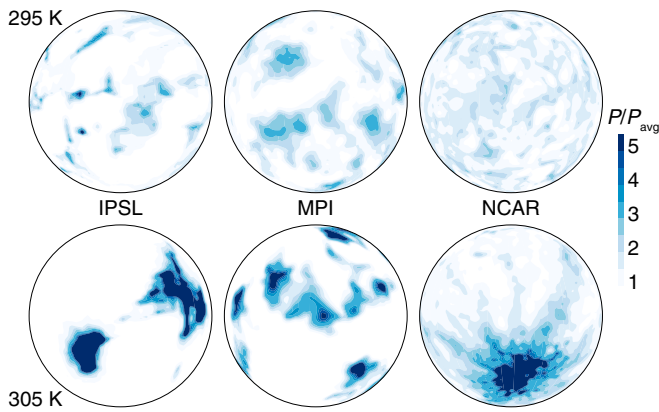
Fig. 1. Monthly precipitation (normalized by its global mean value) predicted by the IPSL, MPI, and NCAR GCMs in RCE simulations forced by an SST of (Top) 295 K and (Bottom) 305 K.
