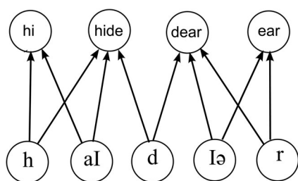
Figure 1. Connectionist network given the sequence /haɪdɪər/.
