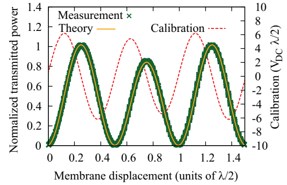
FIG. 2. (Color online) Comparison of the theoretical fringe pattern of a Michelson-Sagnac interferometer with measured output data. The derivative (dashed red line) of the transmitted power serves as calibration of the interferometer output in Fig. 3.
