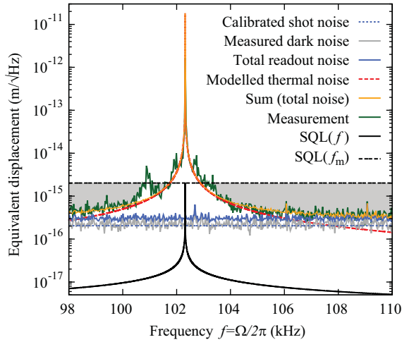
FIG. 3. (Color) Measured (green) and modeled (yellow) noise spectrum of the Michelson-Sagnac laser interferometer containing a \text{SiN}_x membrane at room temperature. The total readout noise (imprecision) has a level of slightly above 3 \times 10^{-16} \text{ m}/\sqrt{\text{Hz}} and is given by the sum of electronic dark noise and shot noise. It lies well below the peak value of the SQL of 2 \times 10^{-15} \text{ m}/\sqrt{\text{Hz}} at the membrane's resonance frequency f_m . For our modeling we assumed all noise sources to be uncorrelated.
