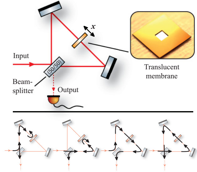
FIG. 1. (Color online) Schematic of the Michelson-Sagnac interferometer. The \text{SiN}_x membrane is aligned such that transmitted and reflected light beams propagate along the same optical axis. The lower row of plots shows the four possible light paths, which interfere at the interferometer output. The inset shows a photograph of the membrane having an area of 1.5 \text{ mm}^2 .
