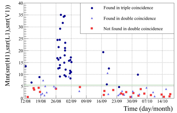
Fig. 7. This plot shows all the successful hardware injection which took place coherently in the three detectors. 93% of those which were above the threshold (expected \text{SNR} \geq 5.5 ) in each detector were detected in triple coincidence by MBTA.
