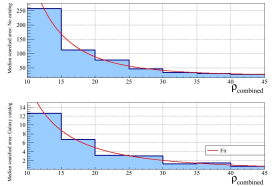
Fig. 5. Sky localization performance as a function of combined signal-to-noise ratio with and without the use of a galaxy catalog (bottom and top panel, respectively). The blue bars indicated the median searched area, in square degrees, in each bin and the red lines depict a fit to these values.
