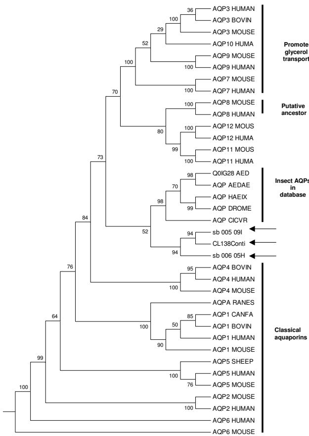
Figure 3 Maximum parsimony tree of 12 aquaporin genes and the three O. arcticus clones (sb_005_09I, CL138 and sb_006_05H07) (arrowed). Accession numbers: Human AQPs 1-12A: P29972, P41181, Q92482, P55087, P55064, Q13520, O14520, O94778, O43315, Q96PS8, Q8NBQ7, Q8IXF9; Mouse AQPs 1-12A (10 is absent): Q02013, P56402, Q8R2NI, P55088, Q9WTY4, Q8C4A0, O54794, P56404, Q9JJJ3, Q8BH11, Q8CHJ2. Bovin AQPs 1, 3, 4: P47865, Q08DE6, O77750. Dog (CANFA) AQP 1: Q9N2J4. Sheep AQP5: Q866S3. Frog AQP (RANES) ( Rana esculenta ): P50501. Insect AQPs: Q0IG28, Q9NHW7: AEDAE: Aedes aegypti (yellow fever mosquito); Q23808: CICVR: Cicadella viridis (green leaf hopper); Q9V5Z7: DROME ( Drosophila melanogaster ) (fruit fly); Q25074: HAEIX ( Haematobia irritans exigua ) (buffalo fly).
