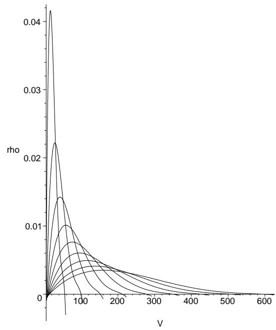
Figure 10: A fit of the spectra described in figure 9 by polynomials of 4th order.
