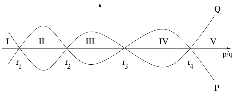
Figure 1: The quaternionic space is basically defined by two fourth order polynomial P(p) and Q(q) which differ only by a total sign. In this figure we have shown the case \kappa > 0 and denoted with I, II, \dots, V the different coordinate regions. The case with negative \kappa corresponds effectively to an exchange of P and Q .
