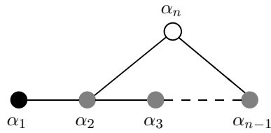
Figure 1. The Dynkin diagram of AE_n with labelling of the simple roots shown. Solid nodes (black and grey) belong to A_{n-1} \equiv \mathfrak{sl}_n which gets enhanced to \mathfrak{gl}_n . Grey nodes mark the common ‘horizontal’ A_{n-2} \equiv \mathfrak{sl}_{n-1} subalgebra.
