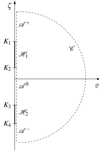
Fig. 1 Illustration of the situation in Weyl coordinates. The event horizons \mathcal{H}_1 and \mathcal{H}_2 of the two black holes are located in the intervals [K_2, K_1] and [K_4, K_3] on the \zeta -axis, respectively. The remaining part of the \zeta -axis corresponds to the rotation axis. In particular, we denote with \mathcal{A}^+ , \mathcal{A}^0 , and \mathcal{A}^- the upper, middle and lower parts of the axis.
