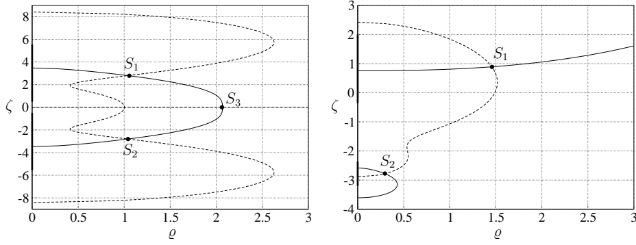
Fig. 2 Singularities of the Ernst potential: The plots show, for two different configurations, curves along which the real part (solid curve) and imaginary part (dashed curve) of the determinant in the denominator of the Ernst potential f vanish. At the intersection points S_1 , S_2 , ( S_3 ), the Ernst potential diverges. The horizons of the two black holes are marked as black lines on the \zeta -axis. Parameters: \phi = \frac{3}{4}\pi , w = 10/3 , w' = 0.3 (left panel) and \phi = -0.1 , w = 1.3 , w' = 0.5 (right panel).
