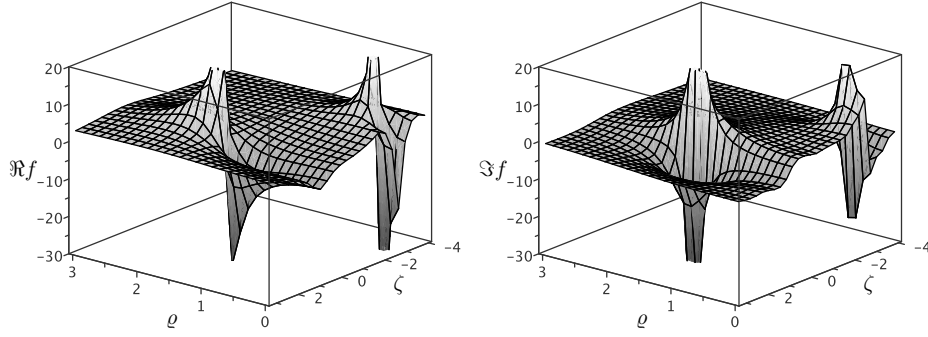
Fig. 3 Singular Ernst-Potential: Real and imaginary part of the Ernst potential f for the example configuration in Fig. 2, right panel.
