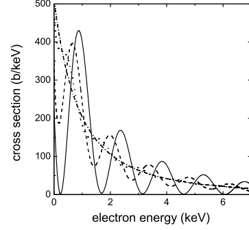
FIG. 2: Energy spectrum of electrons (in a.u.) emitted under the zero azimuthal angle from 7.8 MeV/u \text{Mg}^{11+}(1s) ions colliding with \text{N}_2 . The spectrum is given in the projectile frame. Solid, dash and dot curves corresponds to collisions with the molecules oriented in the target frame under the polar angle \vartheta_M = 0^\circ, 5^\circ and 10^\circ , respectively. For a comparison, dash-dot curve shows the spectrum in collisions with N atoms multiplied by 2.
